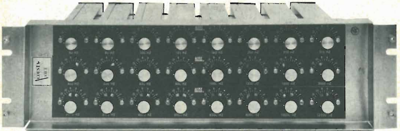
The Altec Lansing 24-filter Acousa-Voice equalizer. Each of the filters can be adjusted in 1-dB steps.
