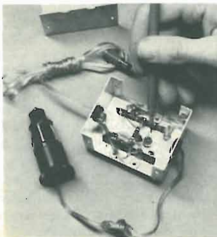
Fig. 3. Model of the converter built by the author. Converter is capable of supplying output currents up to 200 mA. IC is indicated by pencil. Cigarette-lighter plug housing is shown in foreground.
