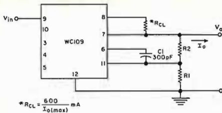
Fig. 2. Diagram of complete voltage converter showing IC and external circuits.
