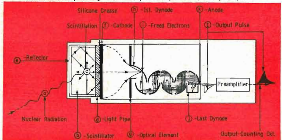
Fig. 4. Schematic representation of gamma scintillation detector showing functional relationship among scintillator, photomultiplier tube, and preamplifier.
