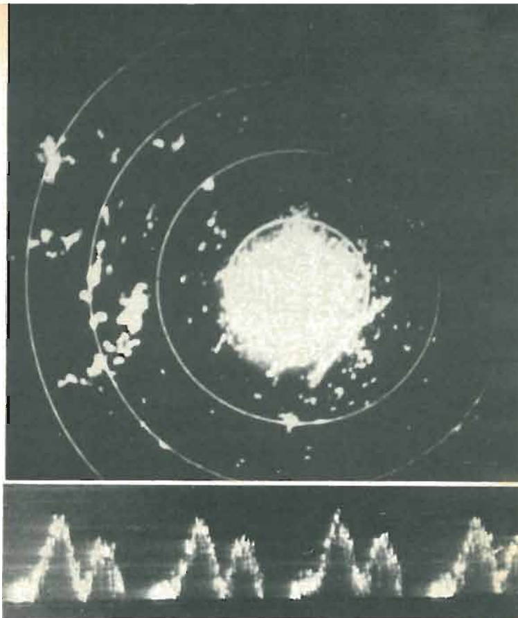
Fig. 2. (Top) A typical plan position indicator display of weather clutter. Magnetic tape recording now makes it possible to continuously repeat storm data to assist the FAA personnel in studying storm signatures' effect on aircraft. (Bottom) Single-sweep "A" scope display of weather formation.
