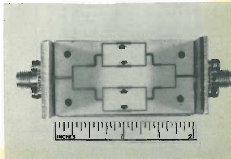
Fig. 5. A 4-to-1 hybrid divider-combiner, which effectively combines four amplifiers (inserted at the arrows) in parallel. These amplifiers may simply be microwave transistors.
