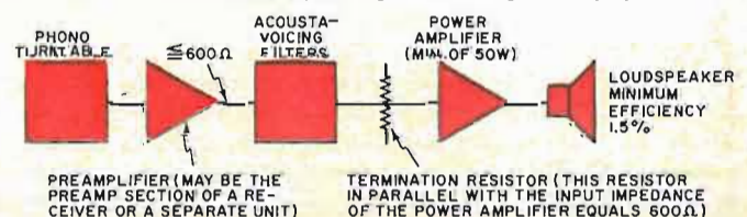
Fig. 6. Installation of equalizing filters in high-fidelity system.
