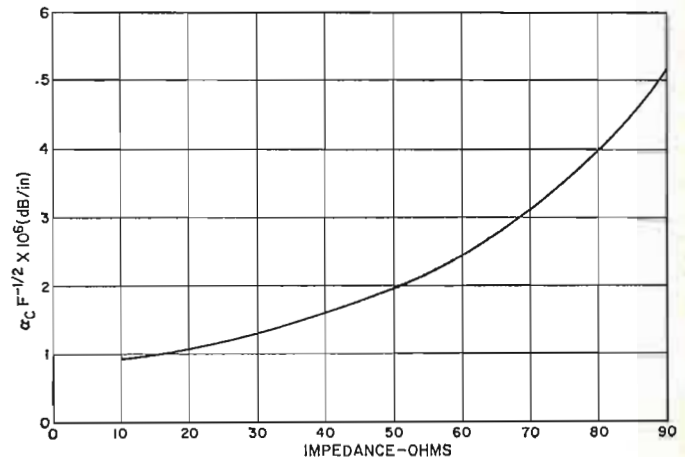
Fig. 4. Attenuation for microstripline at various impedances.
